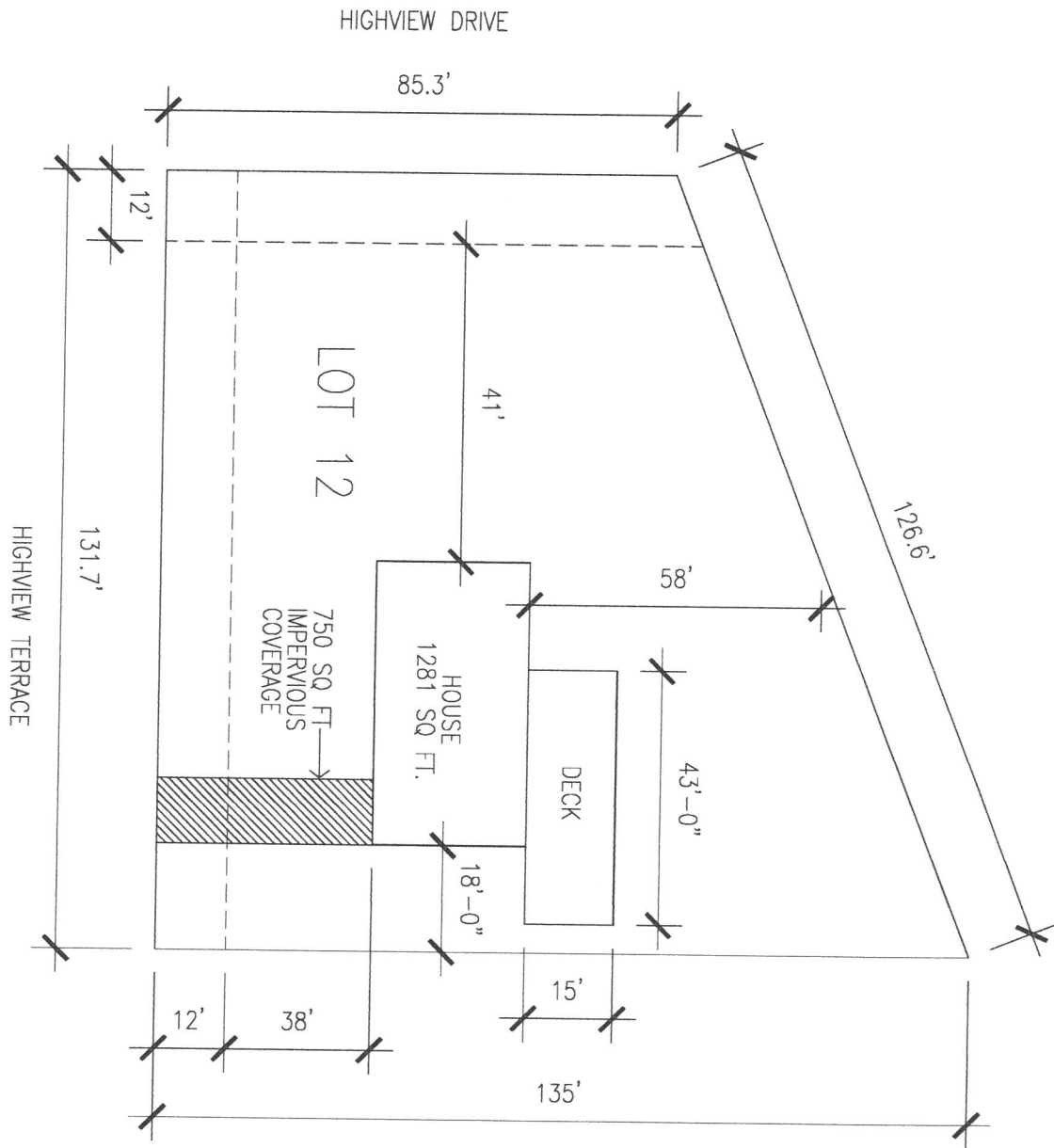
LOT LAYOUT - 3840 HIGHVIEW TERRACE
