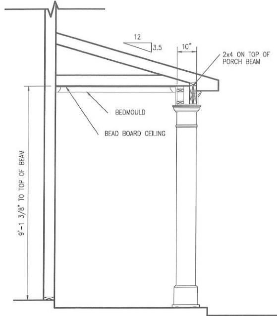
SECTION @ PORCH COLUMN
