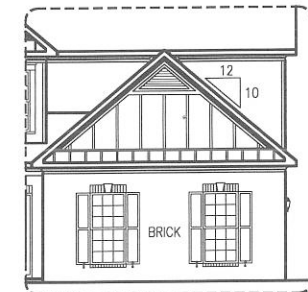
SIDE ENTRY OPTION A117851
