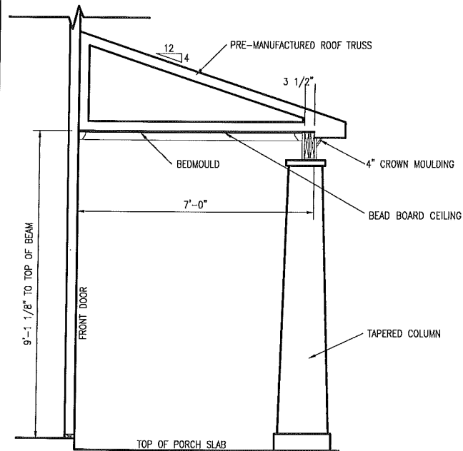
SECTION @ PORCH COLUMN
