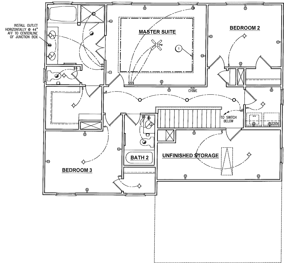
SECOND FLOOR ELECTRICAL PLAN
