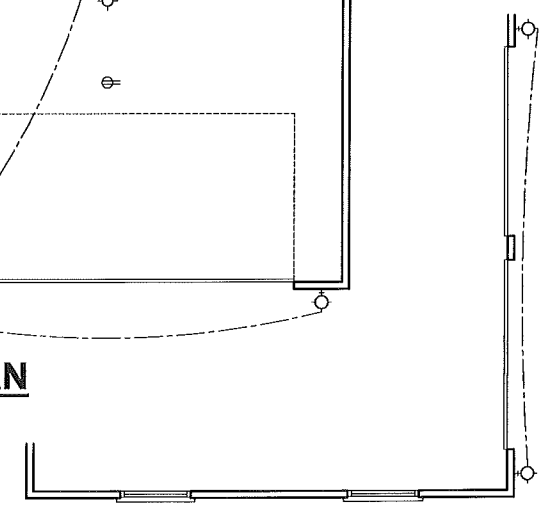
SIDE ENTRY OPTION A117851
