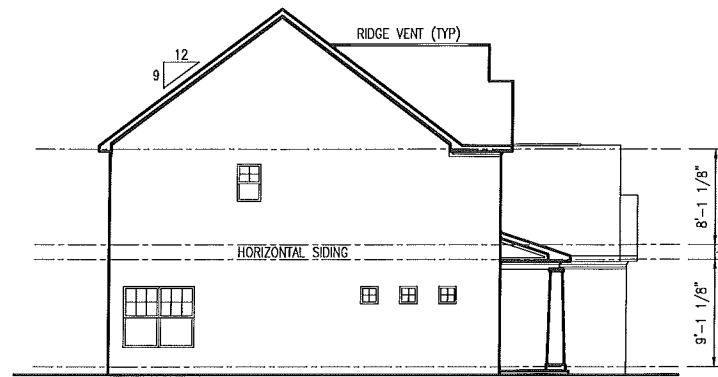
LEFT ELEVATION
