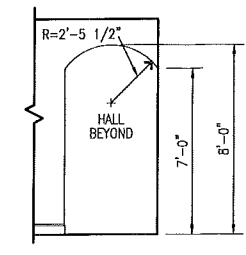
ELEV. @ ARCH
