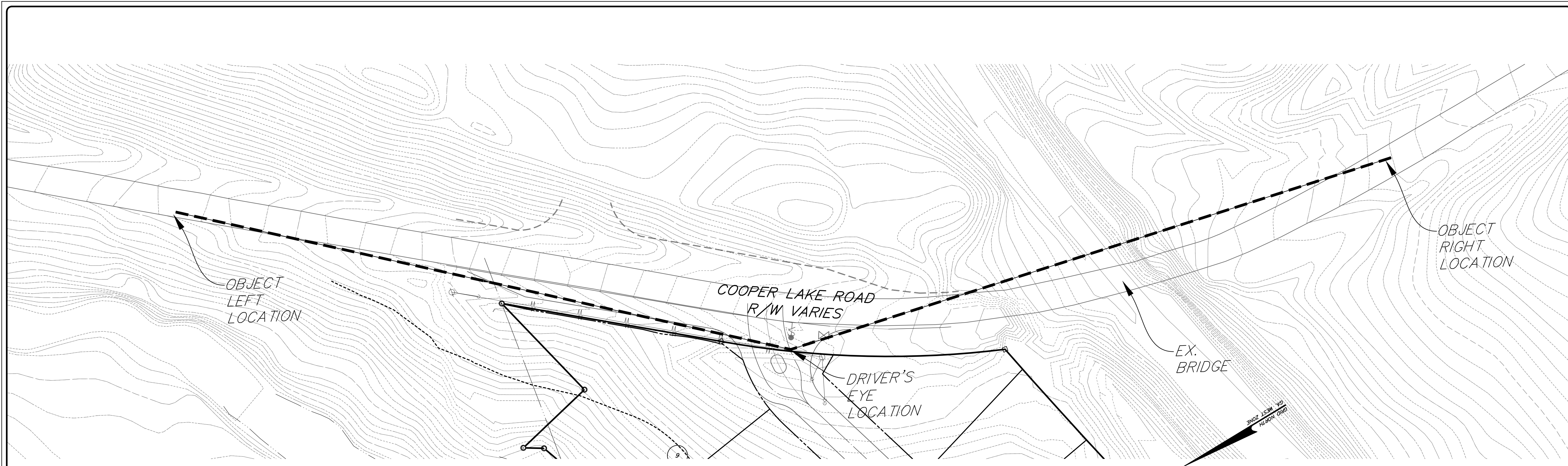
INTERSECTION SIGHT DISTANCE PLAN VIEW SCALE: 1"=40'
