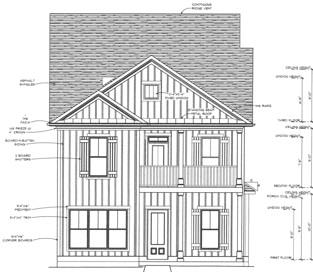
THE "LINTON" FRONT ELEVATION A
