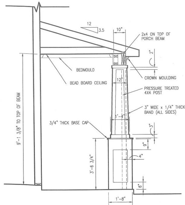
SECTION @ PORCH COLUMN
