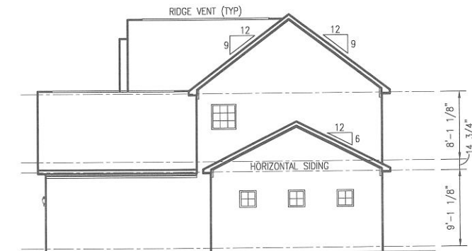
RIGHT ELEVATION W/ TANDEM GARAGE OPTION A114034
