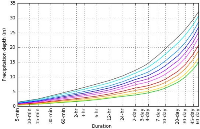
PDS-based depth-duration-frequency (DDF) curves Latitude: 33.8818°, Longitude: -84.5056°
