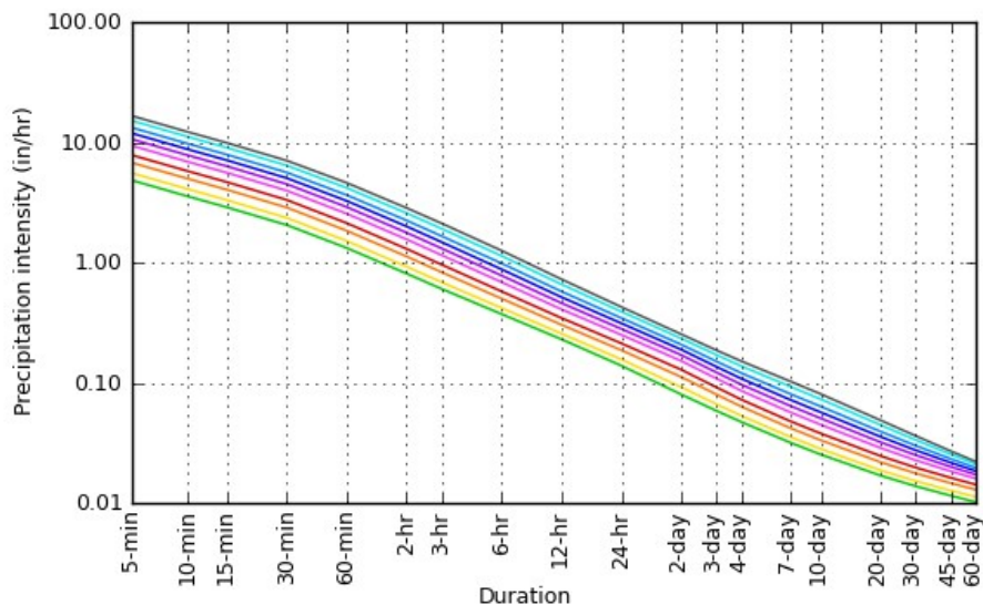
PDS-based intensity-duration-frequency (IDF) curves Latitude: 33.8818°, Longitude: -84.5056°
