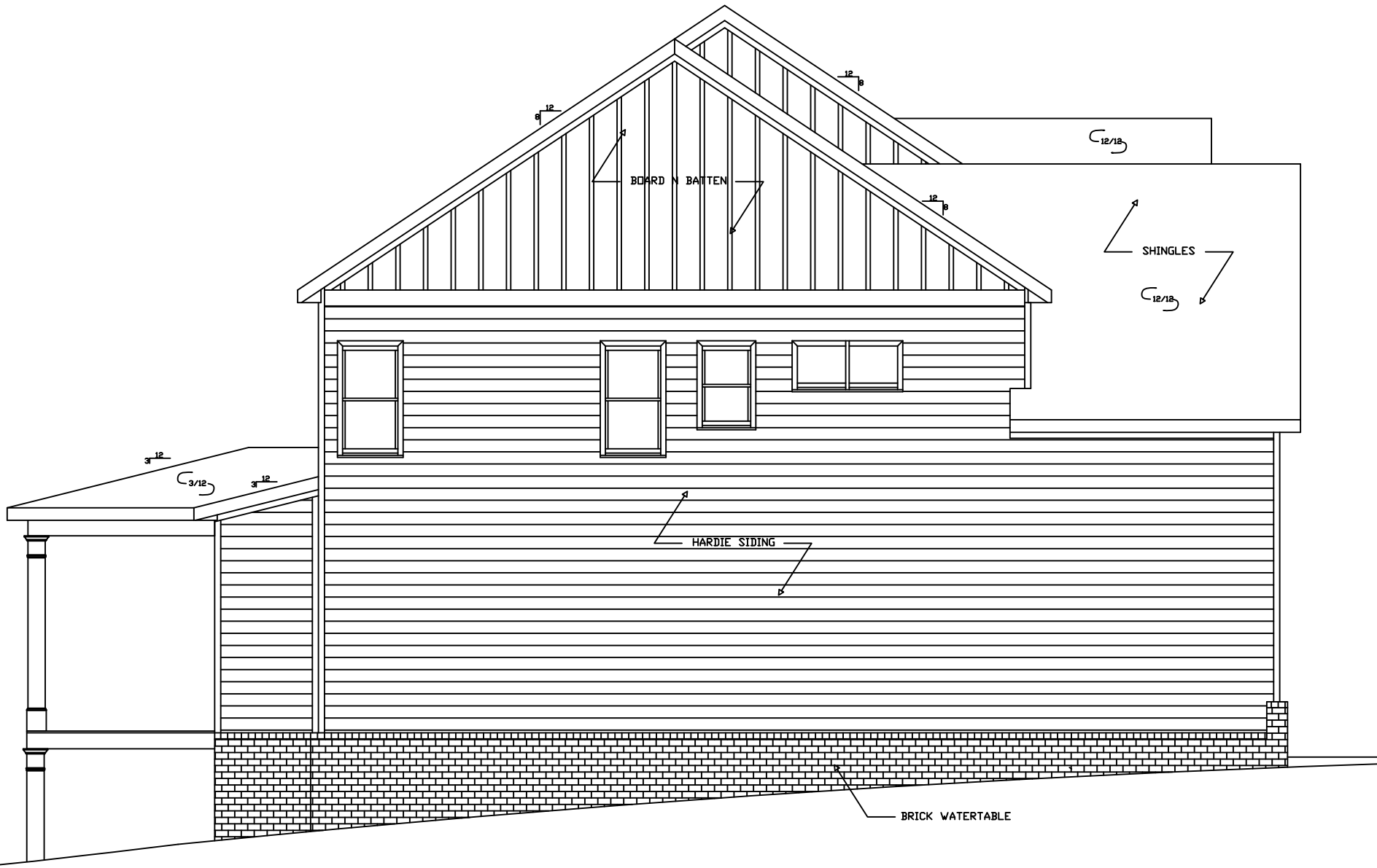
LEFT ELEVATION
