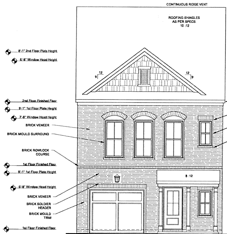
1 CAR FRONT ELEVATION G
