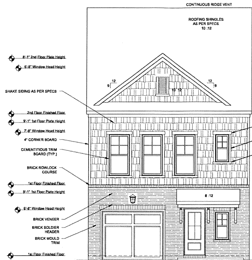
1 CAR FRONT ELEVATION B
