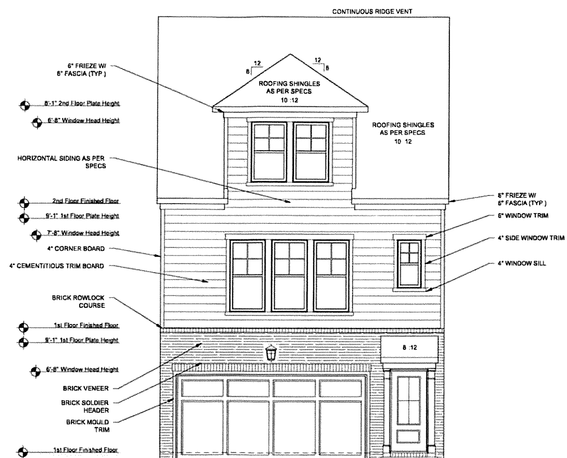
2 CAR FRONT ELEVATION C SCALE: 1/8"=1'-0" (11"x17" SHEET SIZE) SCALE: 1/4"=1'-0" (22"x34" SHEET SIZE)
