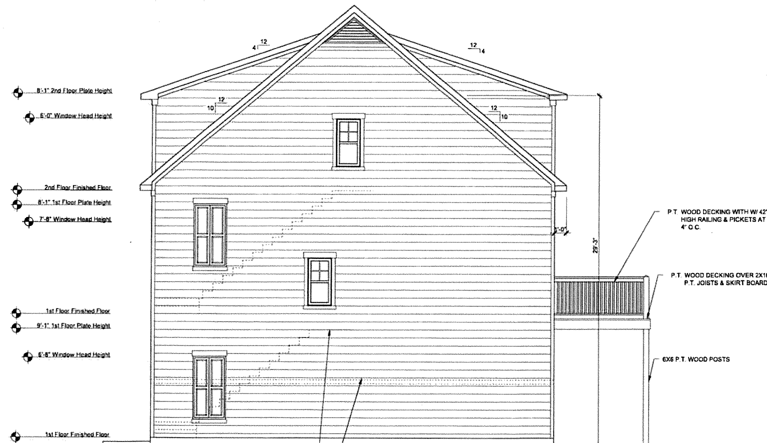
2 CAR RIGHT ELEVATION A SCALE: 1/8"=1'-0" (11"x17" SHEET SIZE) SCALE: 1/4"=1'-0" (22"x34" SHEET SIZE)
