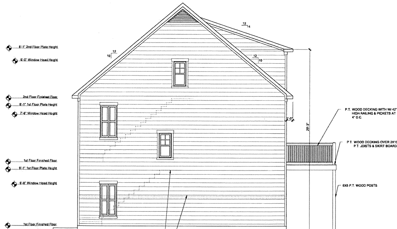
1 CAR RIGHT ELEVATION B
