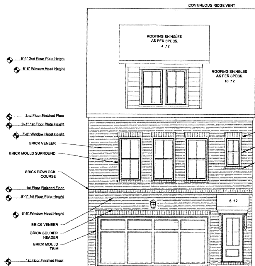
2 CAR FRONT ELEVATION E SCALE: 1/8"=1'-0" (11"x17" SHEET SIZE) SCALE: 1/4"=1'-0" (22"x34" SHEET SIZE)
