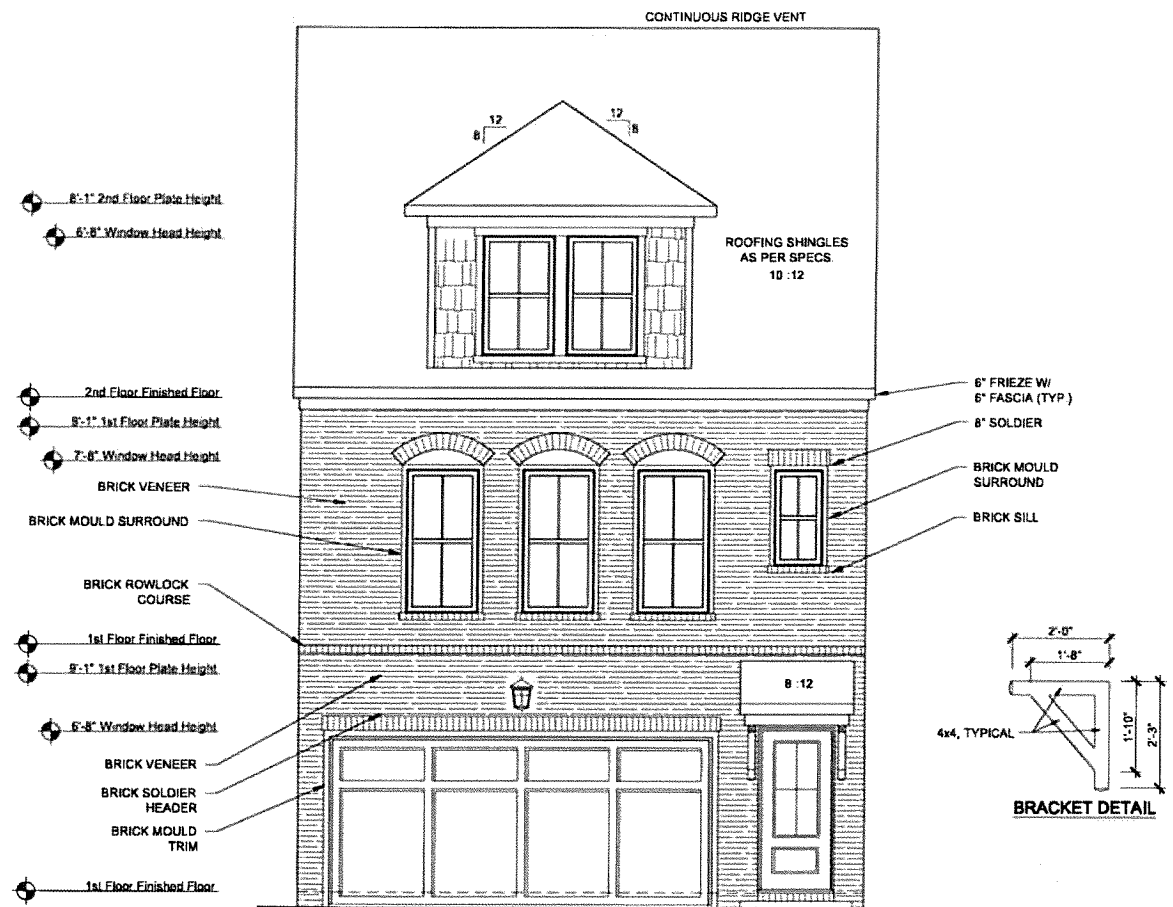
2 CAR FRONT ELEVATION G SCALE: 1/8"=1'-0" (11"x17" SHEET SIZE) SCALE: 1/4"=1'-0" (22"x34" SHEET SIZE)
