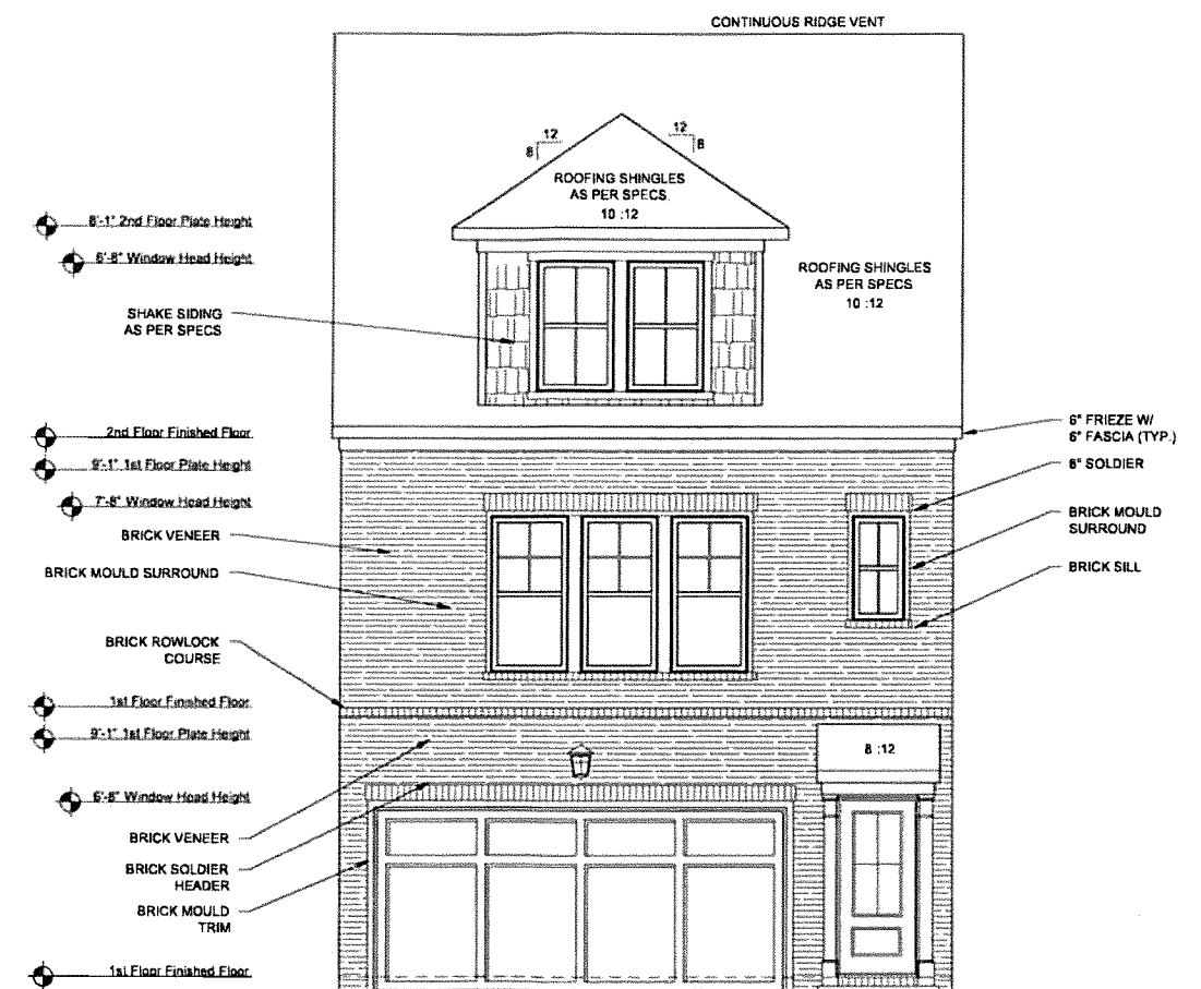
2 CAR FRONT ELEVATION F SCALE: 1/8"=1'-0" (11"x17" SHEET SIZE) SCALE: 1/4"=1'-0" (22"x34" SHEET SIZE)
