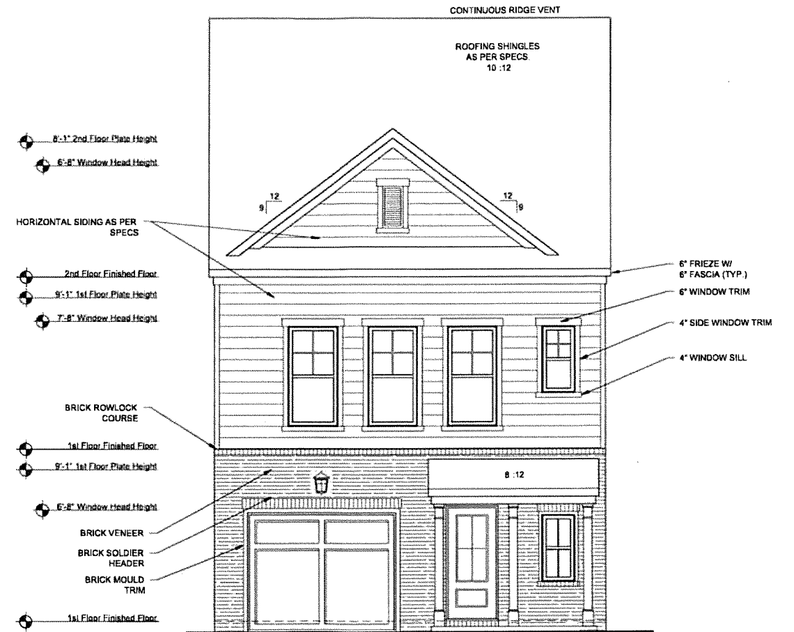
1 CAR FRONT ELEVATION D
