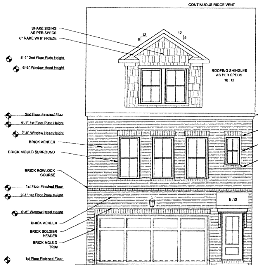
2 CAR FRONT ELEVATION D SCALE: 1/8"=1'-0" (11"x17" SHEET SIZE) SCALE: 1/4"=1'-0" (22"x34" SHEET SIZE)
