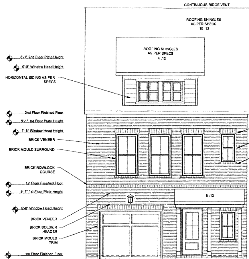
1 CAR FRONT ELEVATION E
