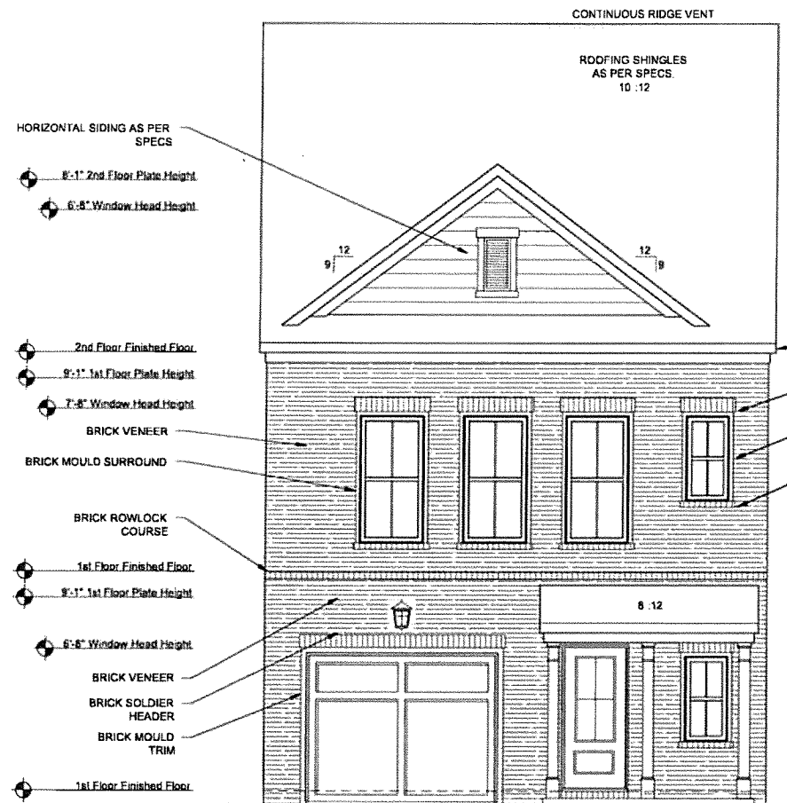
1 CAR FRONT ELEVATION D
