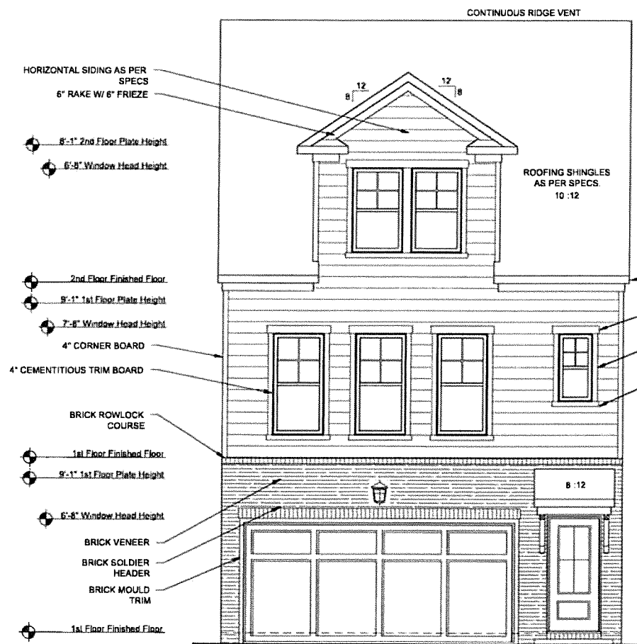
2 CAR FRONT ELEVATION A SCALE: 1/8"=1'-0" (11"x17" SHEET SIZE) SCALE: 1/4"=1'-0" (22"x34" SHEET SIZE)
