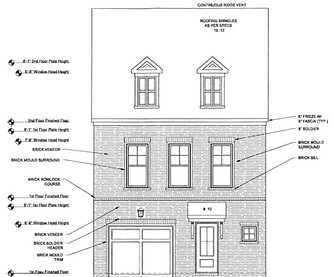
1 CAR FRONT ELEVATION F
