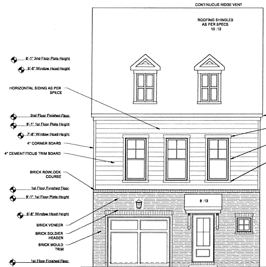
1 CAR FRONT ELEVATION A
