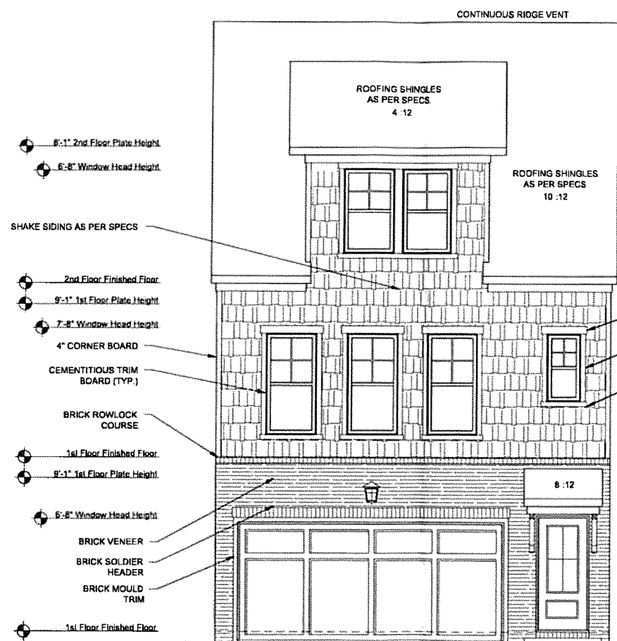
2 CAR FRONT ELEVATION B SCALE: 1/8"=1'-0" (11"x17" SHEET SIZE) SCALE: 1/4"=1'-0" (22"x34" SHEET SIZE)
