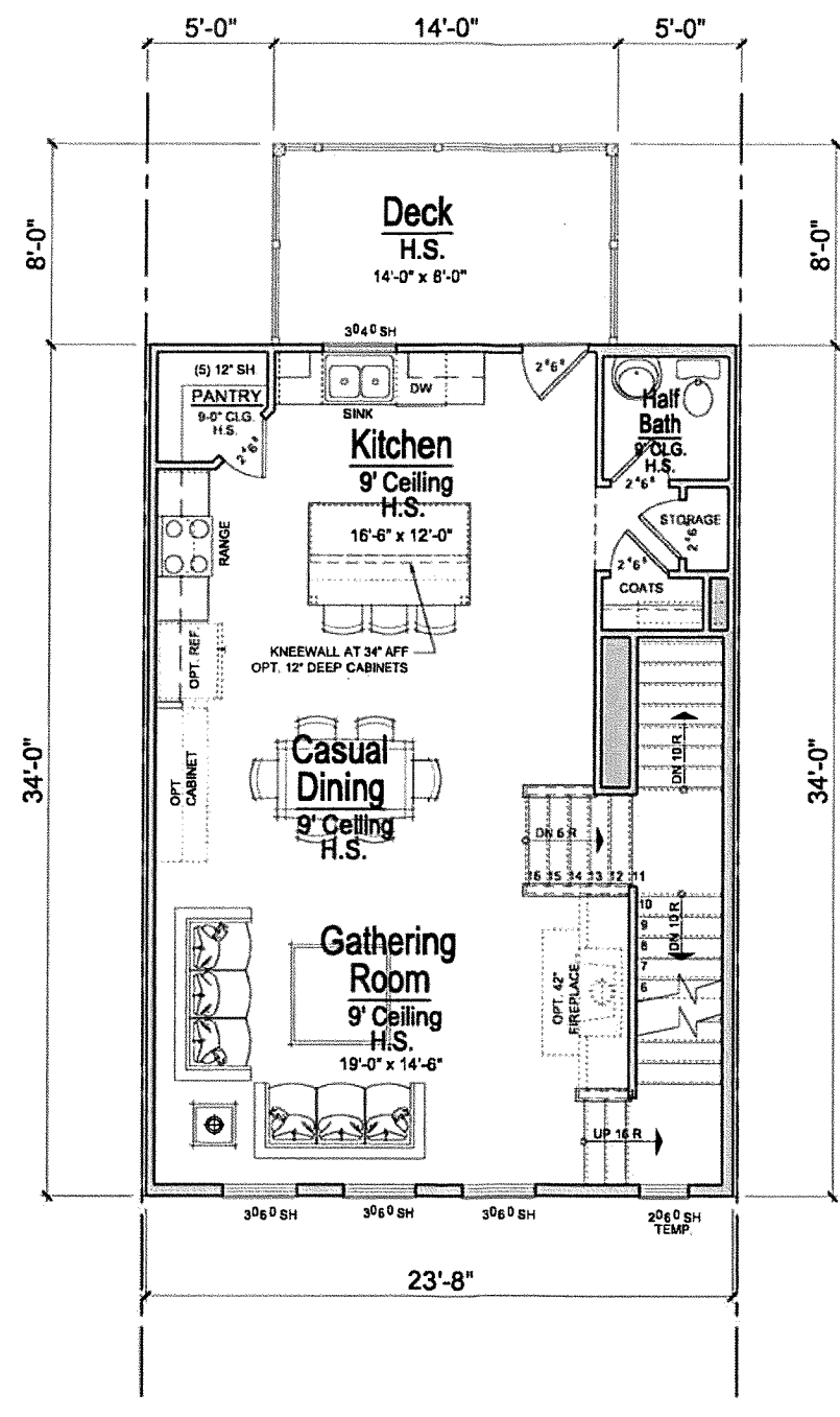
FIRST FLOOR ALTERNATE GATHERING
