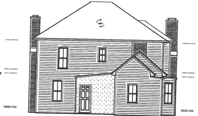
4 REAR ELEVATION
