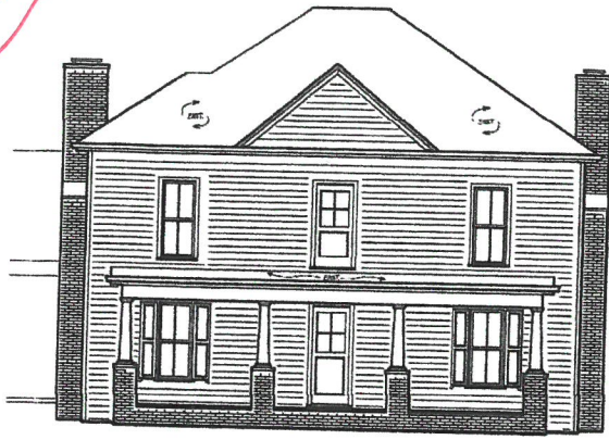
1 FRONT ELEVATION
