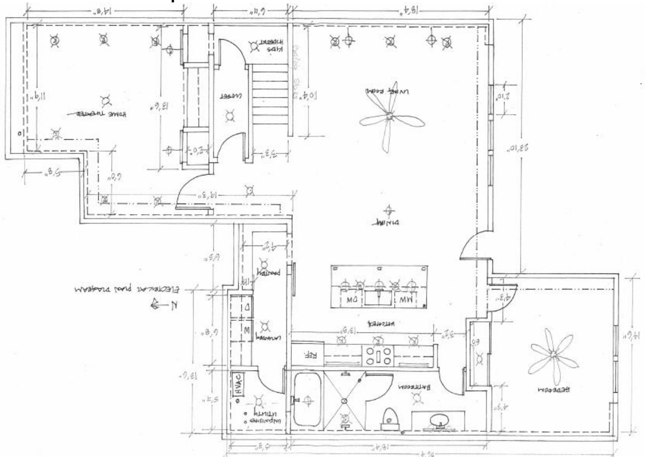
Figure – 4 Proposed Finished Basement Plan
